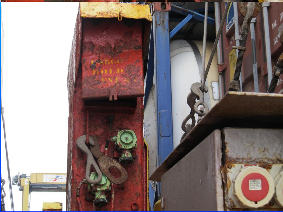
MV MSC Hina: damaged fire dampers, defective manual call points for fire alarm, damaged emergency stop for mooring winch
